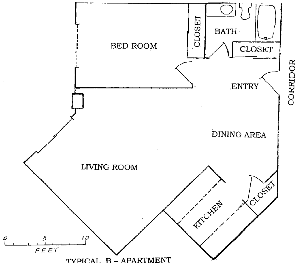
TYPICAL B - APARTMENT THERE MAY BE SLIGHT VARIATIONS IN OTHERS
